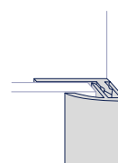
Aluminium click finishing profile (ref. 06430001)
